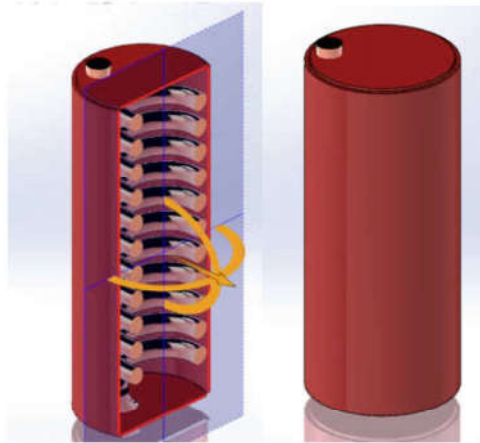
Figure 4. Evaporator Design
